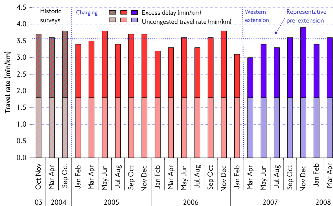
Figure 4.4 Congestion in the western extension zone during charging hours. Moving car observer surveys.
