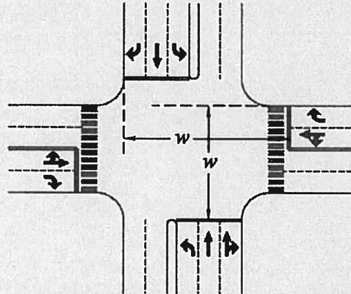
Figure 1 - Intersection Width Measurement for Through Movements
