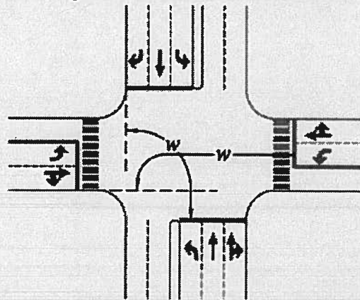
Figure 2 - Intersection Width Measurement for Left-Turn Movements
