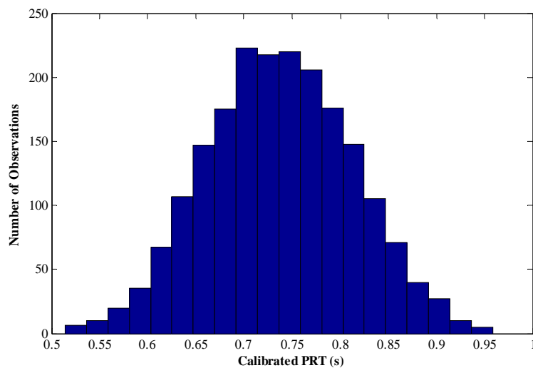
Figure 23. Histograms of model residuals and the calibrated PRT.
