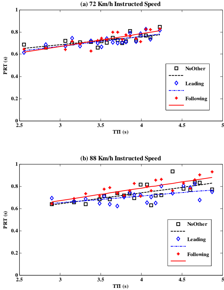
Figure 21. Effect of surrounding traffic on perception-reaction times.
